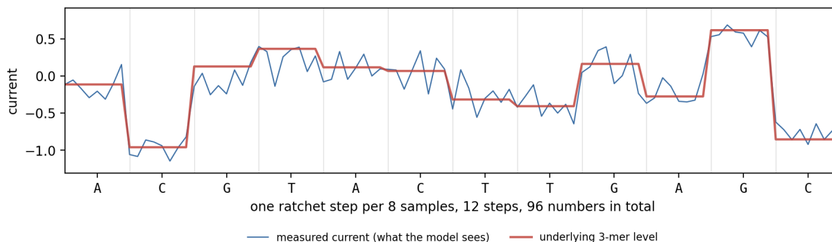
Figure 1: A squiggle from a 12-base strand. The red line is the current each group of bases in the pore produces, the blue line is what actually gets measured.
